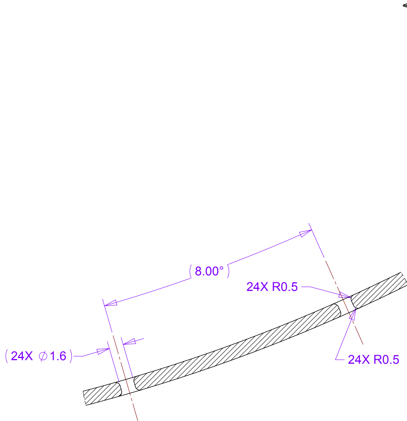
DETAIL A SCALE 4 : 1
