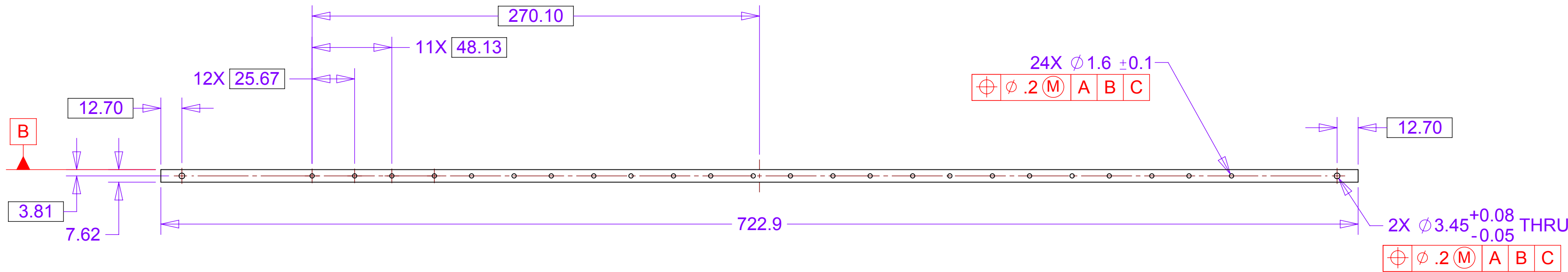
FLAT PATTERN
